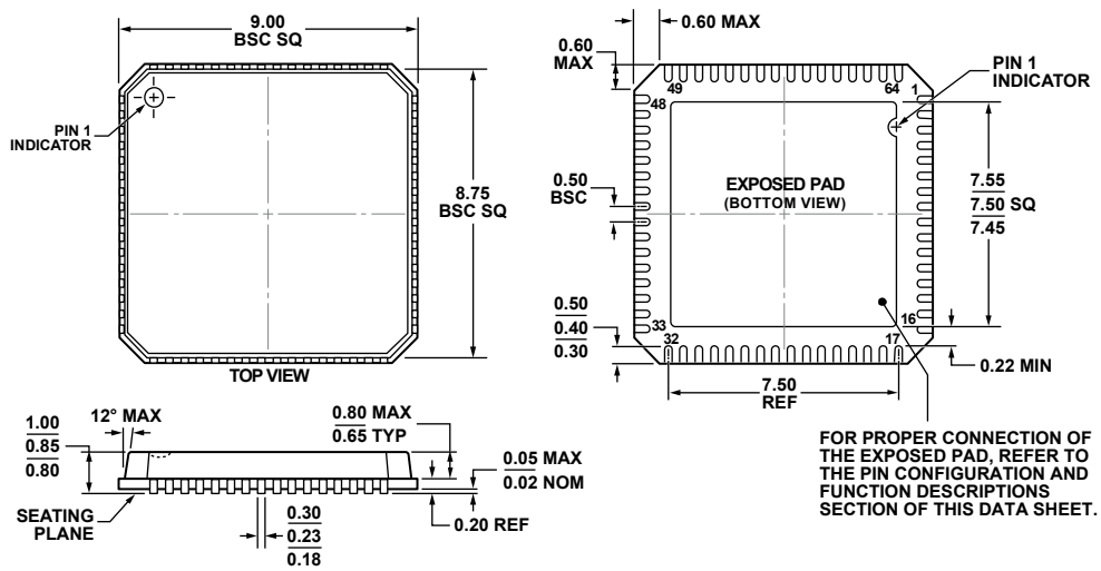
COMPLIANT TO JEDEC STANDARDS MO-220-VMM4 Figure 101. 64-Lead Lead Frame Chip Scale Package [LFCSP_VQ] 9 mm × 9 mm Body, Very Thin Quad (CP-64-6) Dimensions shown in millimeters
