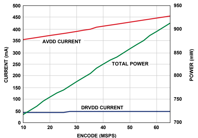
Figure 70. Supply Current vs. f_{SAMPLE} for f_{IN} = 10.3 \text{ MHz} , AD9222- 65
